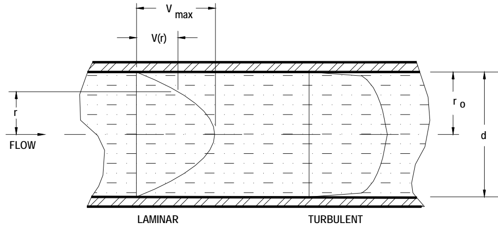
FIGURE 2. PIPE FLOW VELOCITY PROFILES
