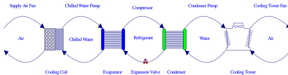
CHILLED WATER SYSTEM WITH WATER COOLED CONDENSER
